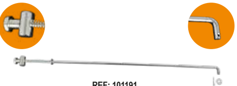
REF: 101191 VARILLA FRENO YAMAHA RX 100/115
