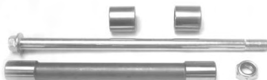
REF: 104250 KIT TIJERA YAMAHA YBR250/FAZER250
